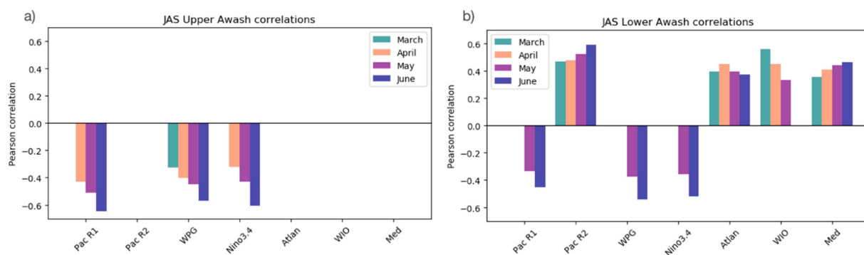
Fig. 10. Correlations of upper Awash (a) and lower Awash (b) JAS rainfall with different SST regions in the month of from March to June to identify potential predictability of JAS rainfall. Correlations are only shown for p < 0.1 .
