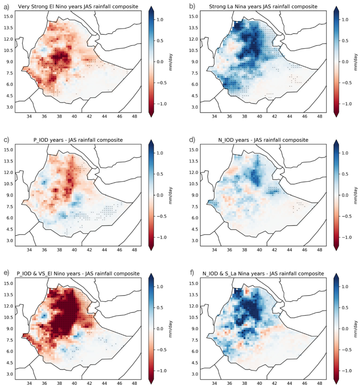
Fig. 7. Composite maps of JAS rainfall for very strong El Nino years (a), strong La Nina years (b), for positive (c), negative IOD years (d), for common years of very strong El Nino & positive IOD years (e) and strong La Nina & negative IOD years (f).
