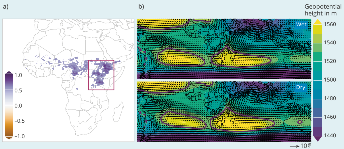
Figure 31: Influence of Atlantic and Mascarene highs on rainfall in the Greater Horn of Africa.
