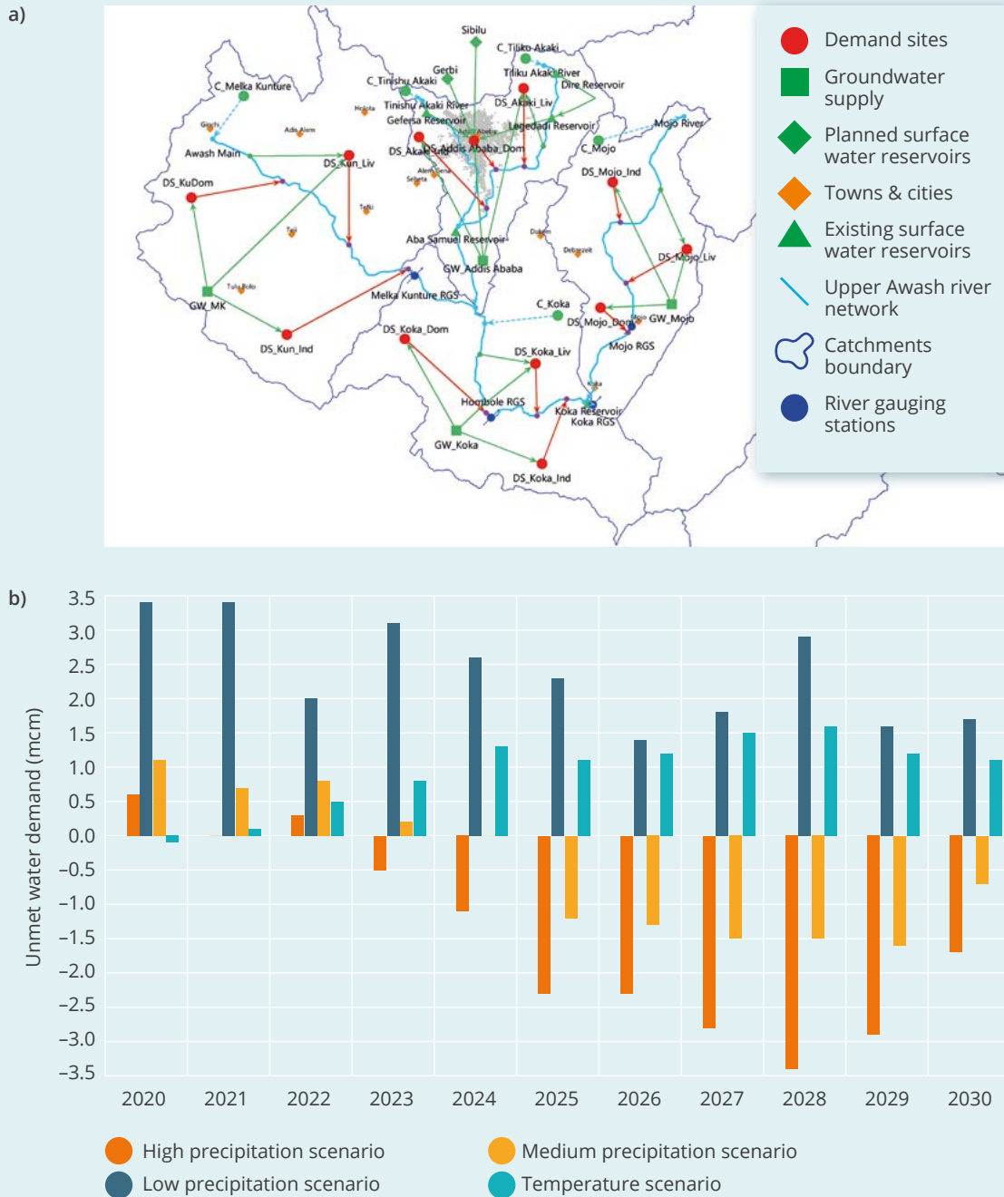
Figure 27: Projected water demand in the upper Awash basin.
