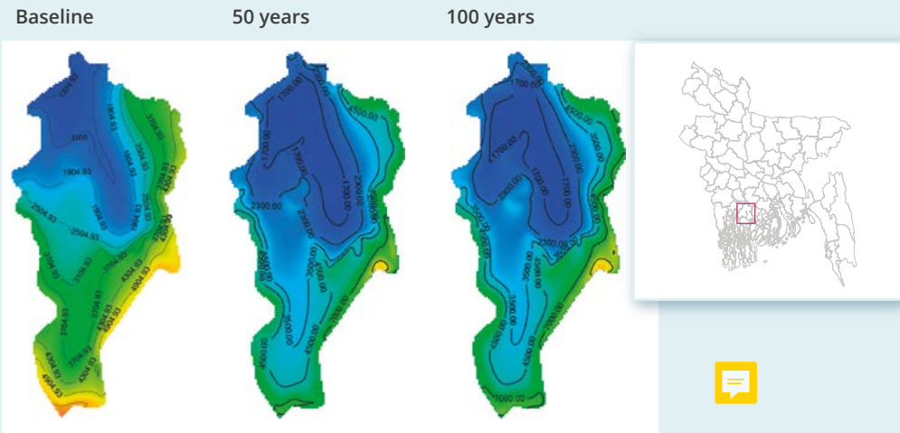
Change in shallow groundwater salinity in response to increase in river salinity
