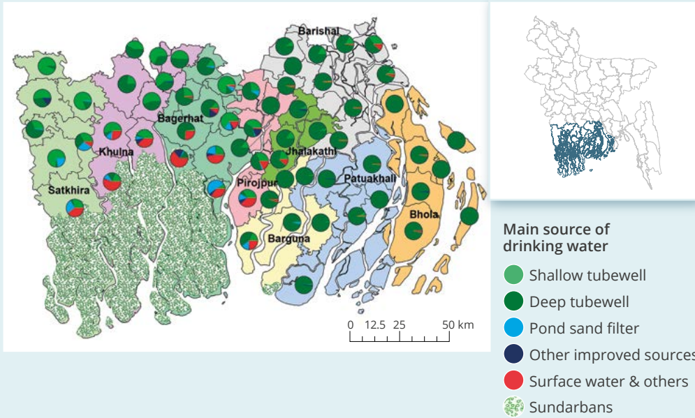
Figure 28: Research shows that salinity in coastal groundwater is a major threat to safe drinking water access.
