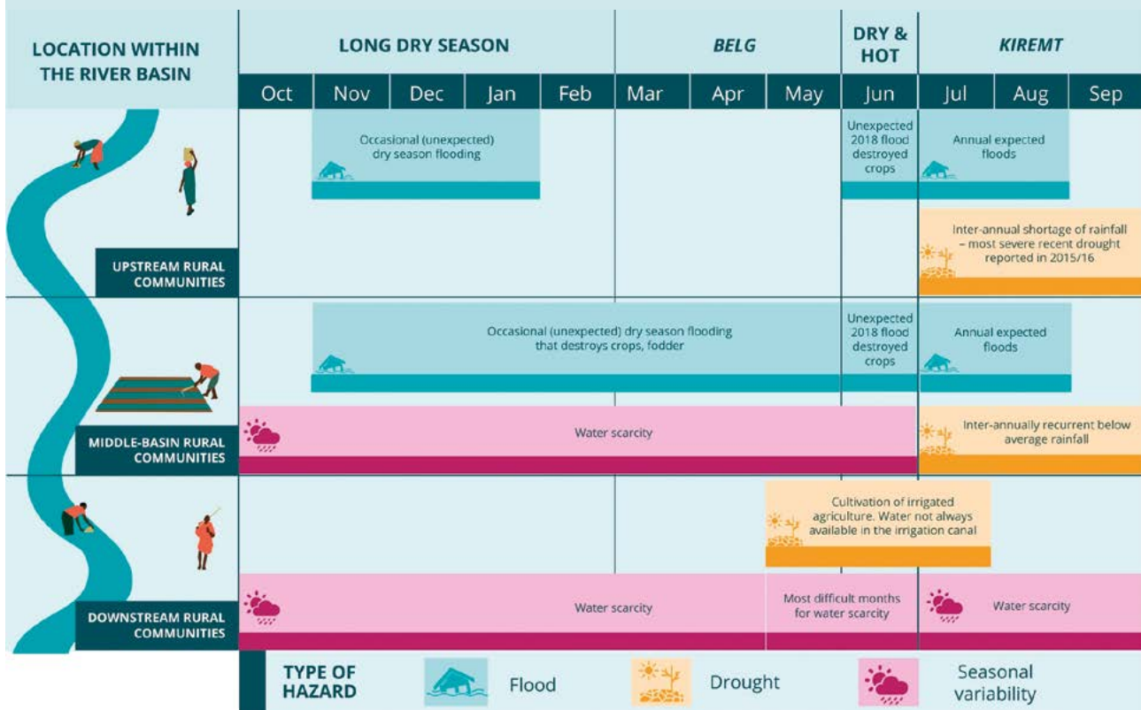
Figure 6: Reported temporal changes in recent extremes and recurrent water and climate-related hazards in the Awash basin , caused by expected and unexpected climate and water resources variability that resulted in exposure and vulnerability to water risk. Water users in the downstream woreda reported rain commonly only falling in July and August and the middle basin user reported rain during kiremt only.
