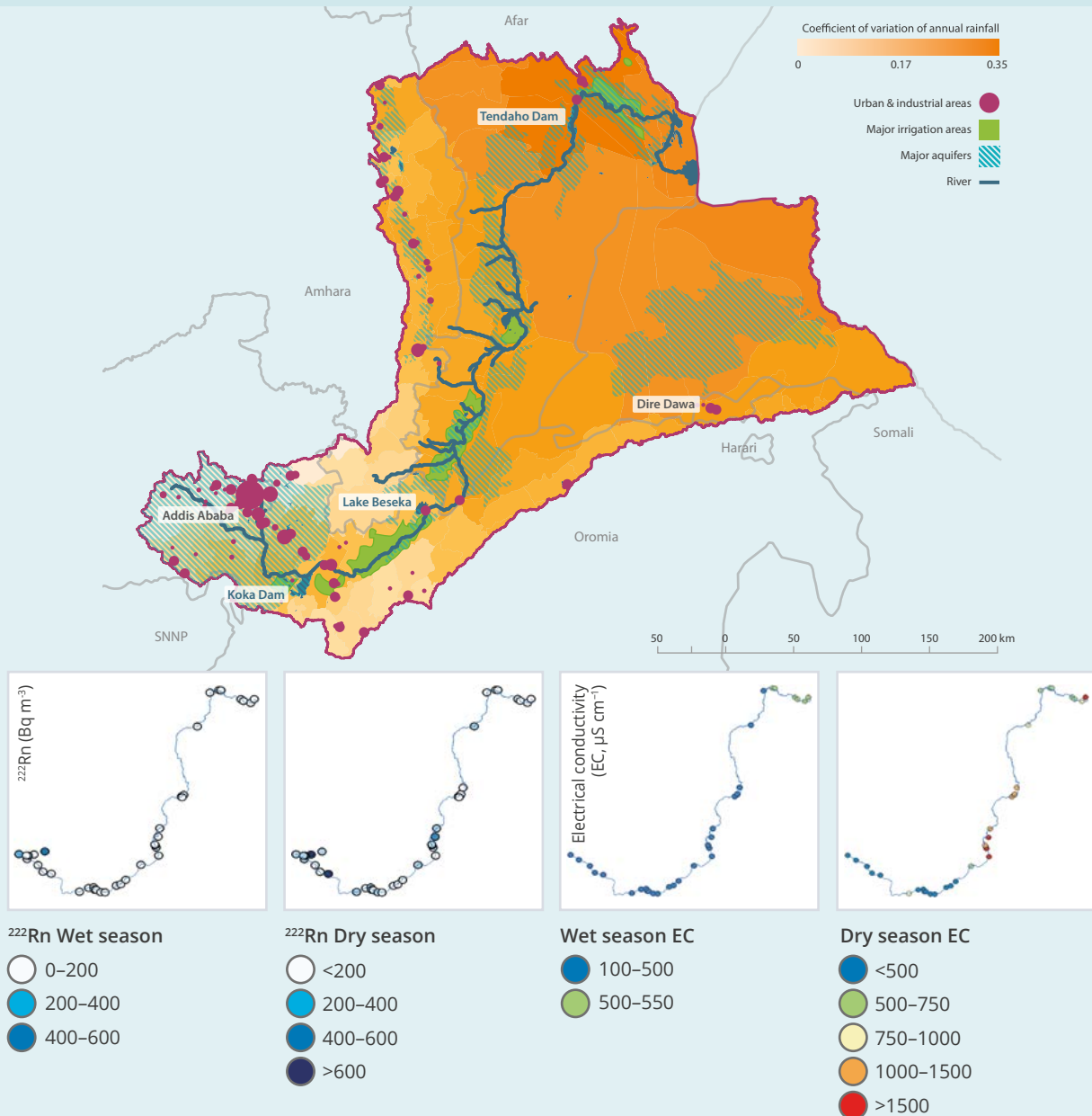
Figure 20: In the Awash river , ^{222}\text{Rn} and electrical conductivity have been used to identify seasonal changes to groundwater influence and water quality.
