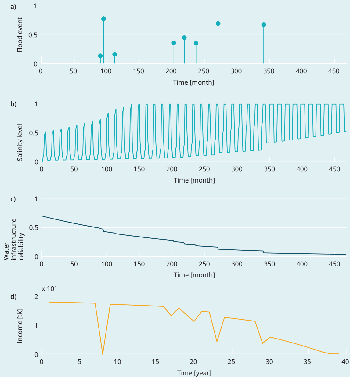
Figure 9: Simulation results from the conceptual human-water dynamical modelling experiment by Borgomeo et al. (2018).
