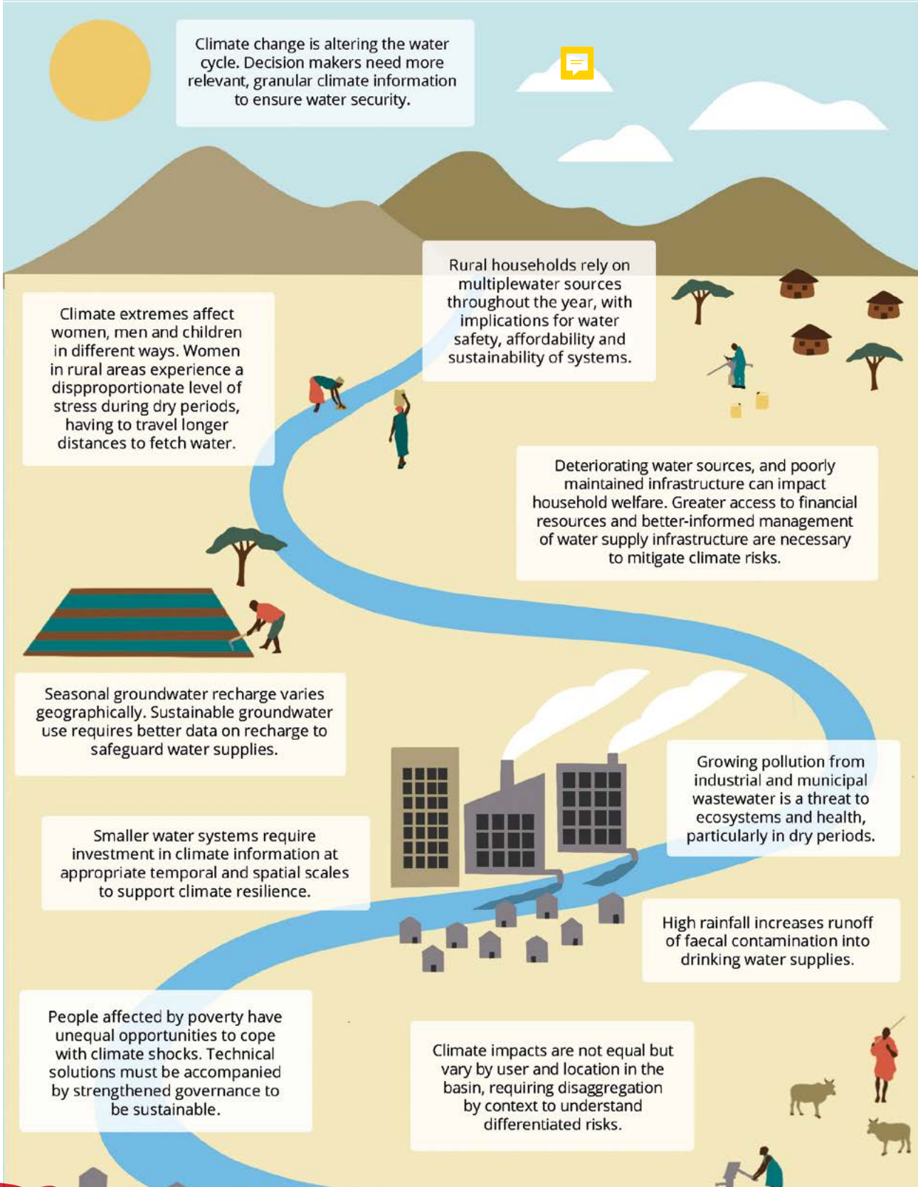
Figure 42: The impacts of climate on water security vary across time and space. They are experienced differently by users across the basin, and are affected by the local hydro-climatic conditions of the area. Improving our understanding of how current and future climate affect water security is critical to building resilience.
