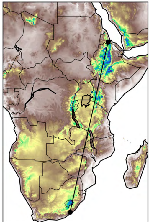
The provision of water vapor is key to understanding rainfall in Africa. In East Africa water vapour transport is dominated by the Turkana Jet (low-level jet stream which present in northwest Kenya). The Turkana Jet accounts for close to 30% of the total water vapour transport from eastern to central Africa across the line shown in right figure (Dr Callum Munday).
